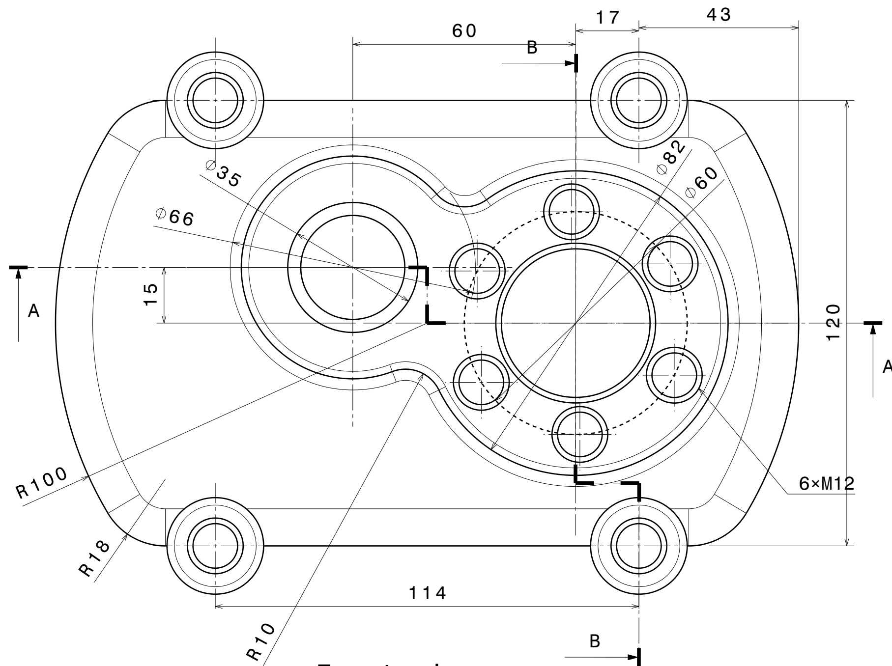
Front view
